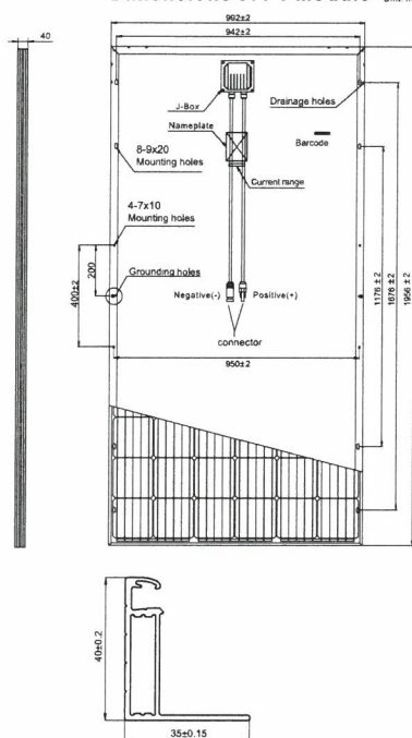
Dimensions of PV Module
